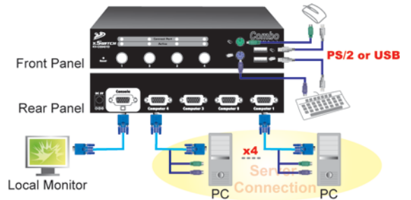
KV-C00401D, KV-P00401D and KV-U00401D Rear Panel View
